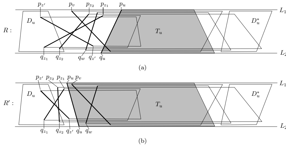
FIG. 3. The movement of the left line l(T_u) of the trapezoid T_u , in order to construct a standard trapezoid representation with respect to u .
