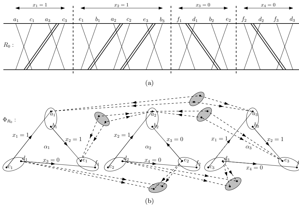
FIG. 6. The NAE-satisfying truth assignment (x_1, x_2, x_3, x_4) = (1, 1, 0, 0) of the formula \phi of Figure 5: (a) an acyclic permutation representation R_0 of P_\phi and (b) the corresponding transitive orientation \Phi_{R_0} of P_\phi .
