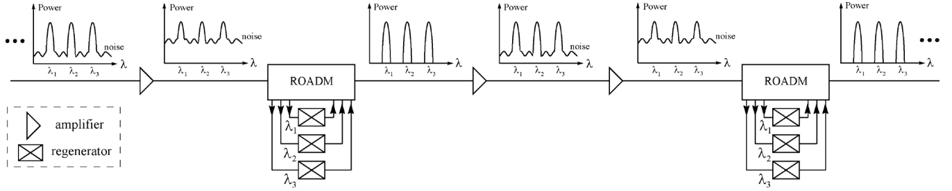
Fig. 1. Simplified optical network: Amplifiers introduce noise into the signal, which needs to be regenerated after at most d = 3 hops. When the signal is regenerated through an ROADM, a different regenerator is needed for each wavelength.
