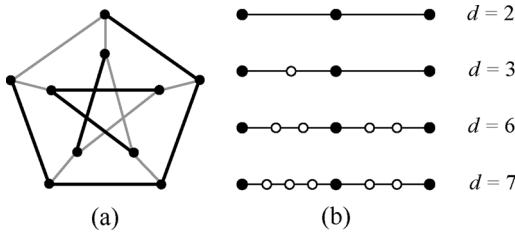
Fig. 2. (a) Two-coloring of the edges of the Petersen graph (gray and black) such that each monochromatic component is a path of length at most 5. (b) Construction of the lightpaths from a path of length 2 for several values of d , in the proof of Theorem 1. Full dots correspond to vertices of the VERTEX COVER instance (called black in the proof).
