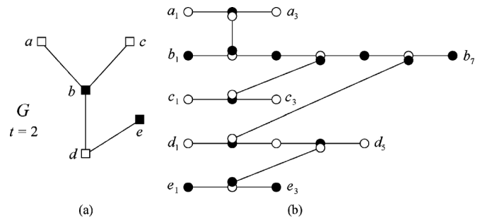
Fig. 3. Reduction from VC to (2, 1) -RL in the proof of Proposition 5. (a) Instance G of VC, where the squares indicate a vertex cover. (b) Instance of (2, 1) -RL constructed from G with |V(G)| + |E(G)| lightpaths, where for simplicity the first and last edge of each lightpath are not depicted. Black vertices correspond to regenerators associated with a vertex and a lightpath, defining a feasible solution for this instance.
