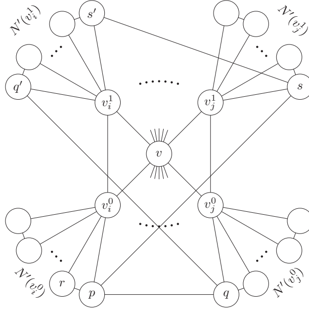
Figure 4: The regularity of the friendship graph G .
